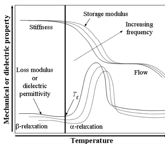
Figure 2 Changes in dielectric and mechanical properties of materials around and above glass transition. In dielectric measurements, dielectric permittivity increases rapidly and shows a dielectric peak above glass transition temperature, while mechanical properties show a drop in storage modulus and a peak of loss modulus at temperature above T_g . The \alpha -relaxation as measured by dielectric (DEA) and dynamic-mechanical (DMA) analysis can be identified from changes in dielectric and mechanical properties around and above glass transition. Appearance of \alpha -relaxation suggests some changes in molecular mobility in the materials [6, 52].
