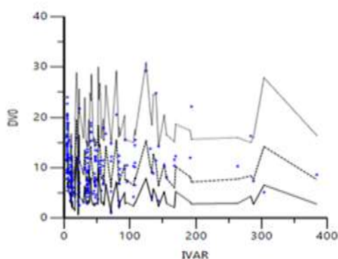
Figure 3 Visual predictive check (VPC) of the final model.
