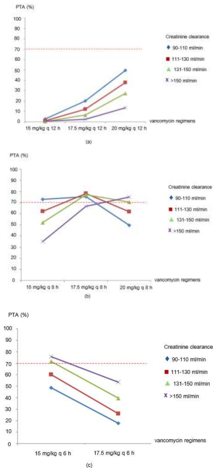
Figure 4 PTA of simulated vancomycin dosing regimens by CL_{cr} category that achieved the target AUC/MIC ratio of 400-600, assuming a MIC of 1 mg/L
