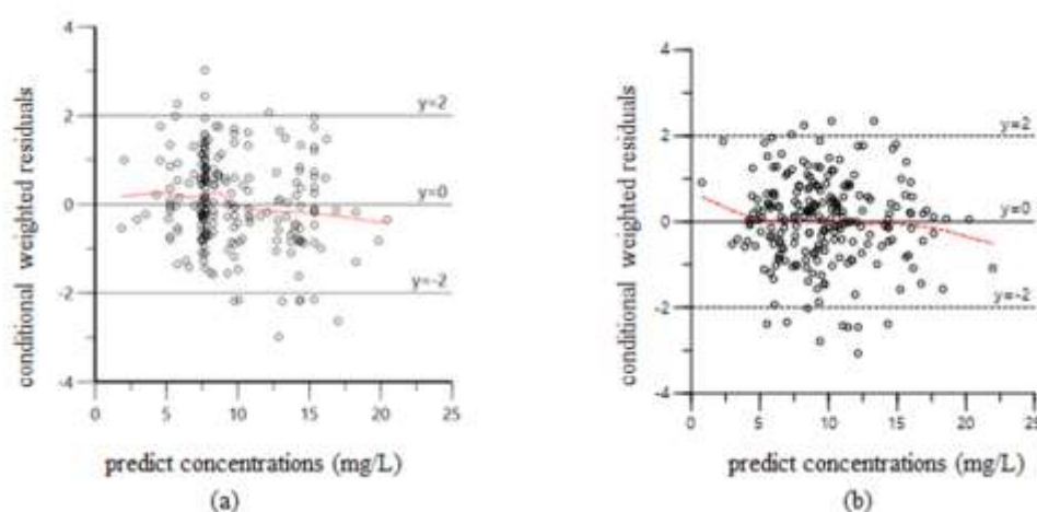
Figure 2 Conditional weighted residuals versus predict concentrations: (a) Base model (b) Final
