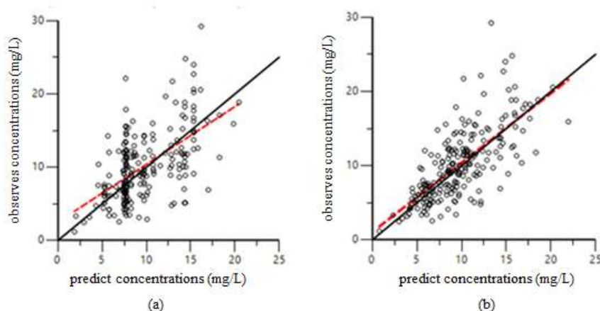
Figure 1 Scatter plot of the observed concentration versus predicted concentrations: (a) Base model (b) Final (covariate) model
