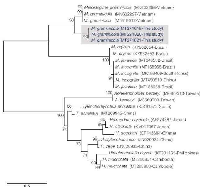
Figure 5 Phylogenetic reconstruction based on 18S-ITS1-5.8S regions of Meloidogyne graminicola isolated from Sam Khok's rice field, Pathum Thani province, Thailand and some other plant-parasitic nematodes in rice. Numbers beside branches represent ML bootstrap support values \geq 70\% . Scale bar represents substitutions per nucleotide position. NCBI accession numbers are listed behind the species names
