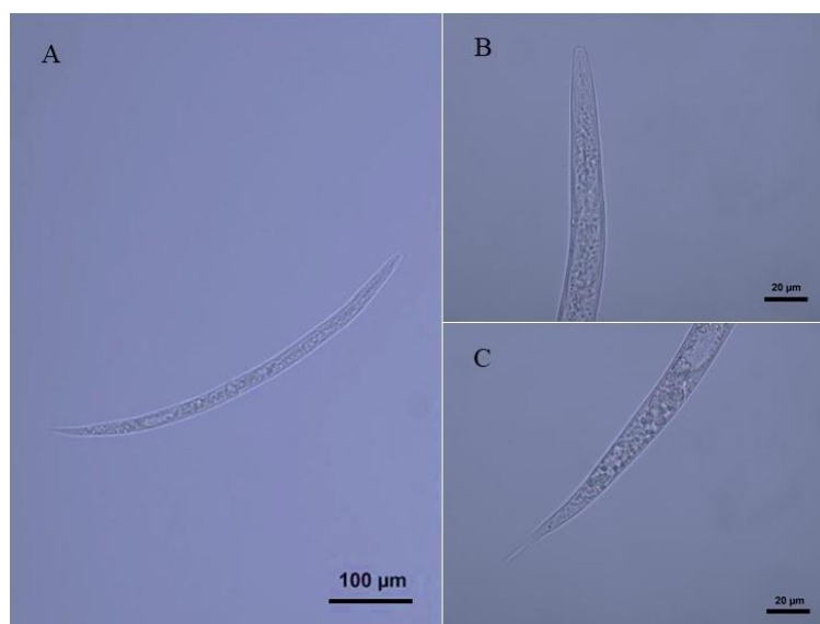
Figure 3 Photographs of second stage juvenile of Meloidogyne graminicola , (A) Whole body (100x); (B) Anterior region (1,000x); (C) Posterior region (1,000x)
