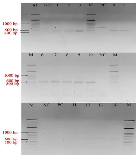
Figure 4 Agarose gel electrophoresis of PCR-amplified DNA of Meloidogyne graminicola , isolated from Sam Khok district, Pathum Thani province, Thailand, by using primers rDNA2/rDNA1.58s (lane no. 1–3), C_2F_3/1108 (lane no. 4–10) and SCAR-MgFW/ SCAR-MgRev (lane no. 11–14). (M) 100+bp DNA marker; (NC) negative control without DNA template; (PC) positive control with DNA template of Meloidogyne enterolobii
