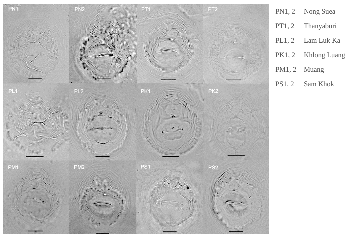
Figure 2 Perineal pattern analysis of root-knot nematodes collected from rice fields of Pathum Thani province, Thailand. Scale bars= 20 \mu m
