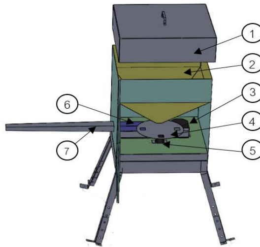
Figure 1 Components of an automatic fish feeder
