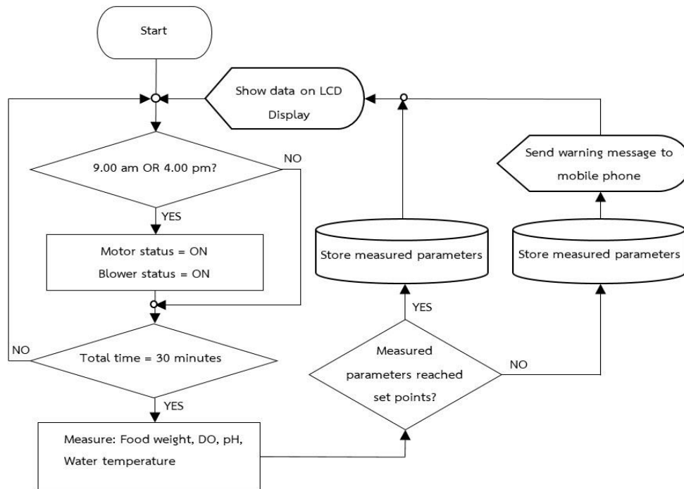
Figure 3 Flowchart of system controller
