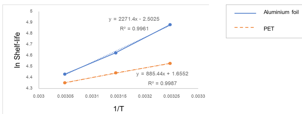
Figure 3 Shelf-life plot crispy cricket in different packages (PET and Aluminium foil).
