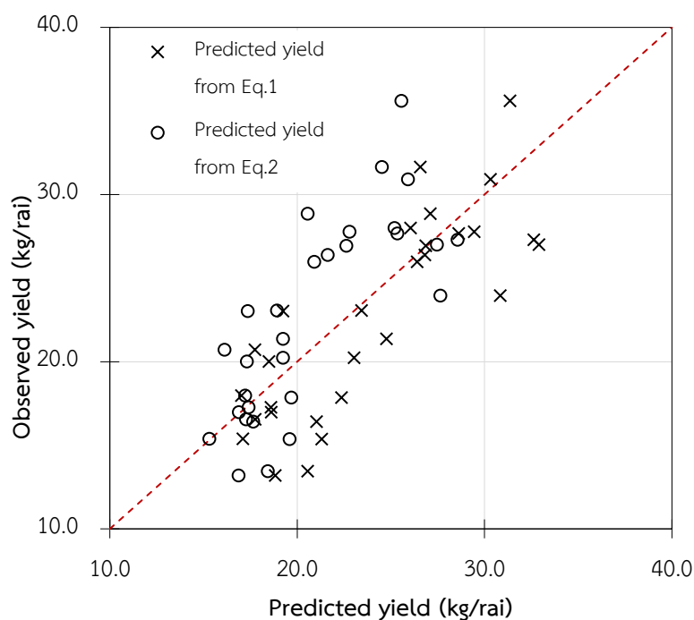
Figure 5 The relationship between observed monthly yield and predicted monthly yield in 2017-2019 from equation 1 (Yield (kg/rai) = 59.02 – 179.37NIR + 40.81NDVI monthly ) and equation 2 (Yield (kg/rai) = 58.12 – 104.70NIR monthly ). The 1:1 reference line is represented by the red dotted line
