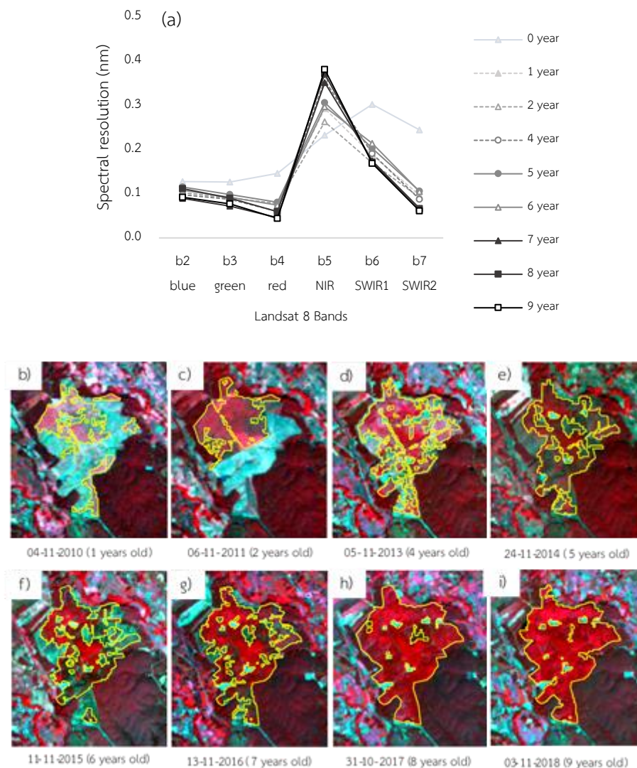
Figure 4 Spectral signature of para rubber in different age (a) and the rubber plantation identification from false-color Landsat 8 OLI of 1-year-old (b) 2-year-old (c) 4-year-old (d) 5-year-old (e) 6-year-old (f) 7-year-old (g) 8-year-old (h) and 9-year-old (i) of rubber in Thoen, Lampang
