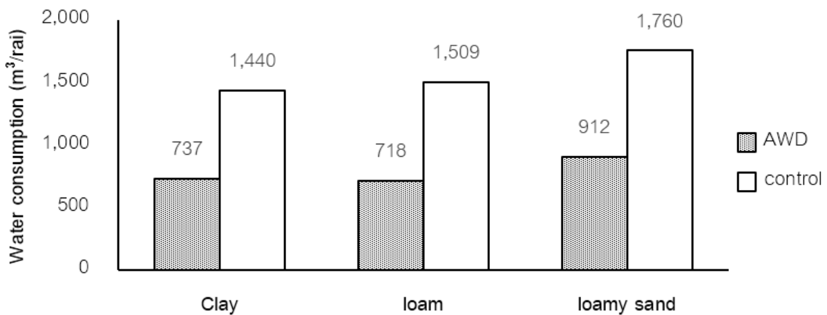
Figure 1 Water consumption of wetting and drying irrigation regime (AWD) comparison with continuous flooding (control) of different soil texture
