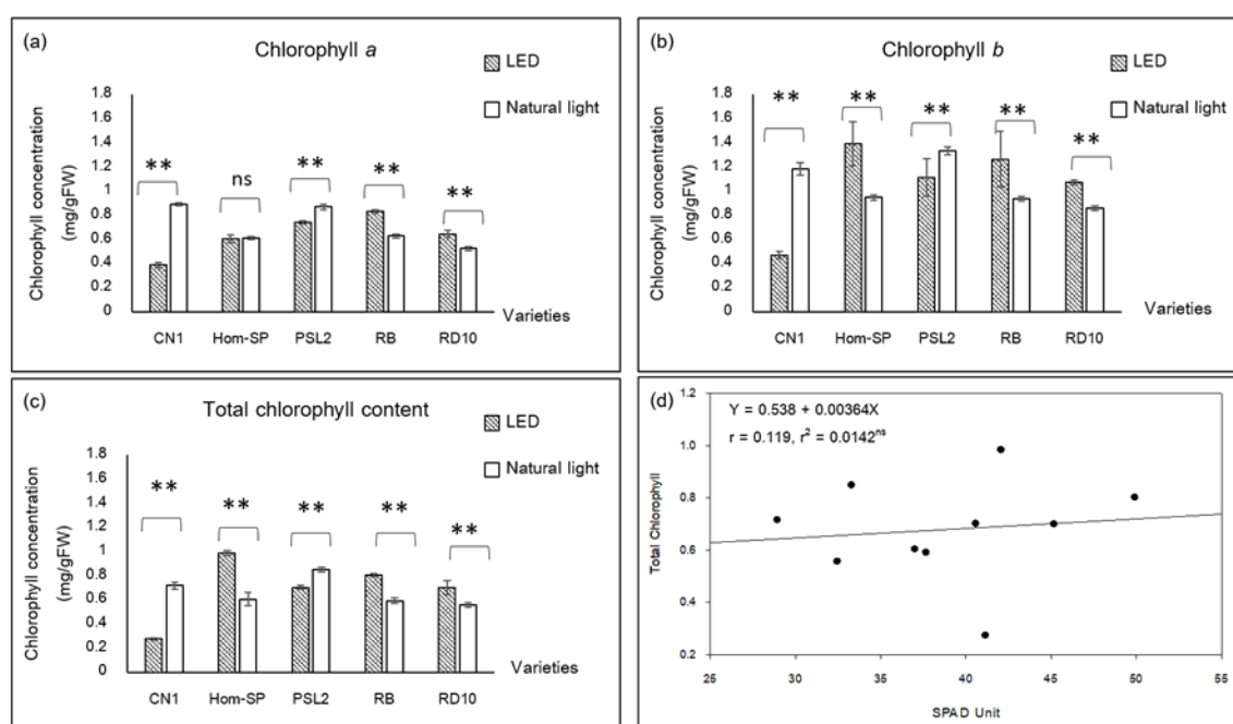
Figure 3 Chlorophyll a (a), chlorophyll b (b), total chlorophyll content (c), and relationship between SPAD values and total chlorophyll content (d) of different rice varieties grown under LED and natural light treatments. All data are the mean \pm standard error of five replications. ** indicates significant differences at p < 0.01 between the values in LED and natural light treatments. The coefficient of variation (CV %) for Chlorophyll a, b, and total chlorophyll is 29.51%, 30.50%, and 31.52%, respectively.
