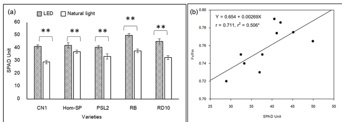
Figure 2 SPAD value at tillering stage of five rice varieties grown under LED and natural light (a), and correlation between SPAD values and Fv/Fm of five rice varieties at tillering stage. All data are the mean \pm standard error of five replications. ** indicates significant differences at P < 0.01 between the values in LED and natural light treatments. The coefficient of variation (CV %) for SPAD is 17.17%.
