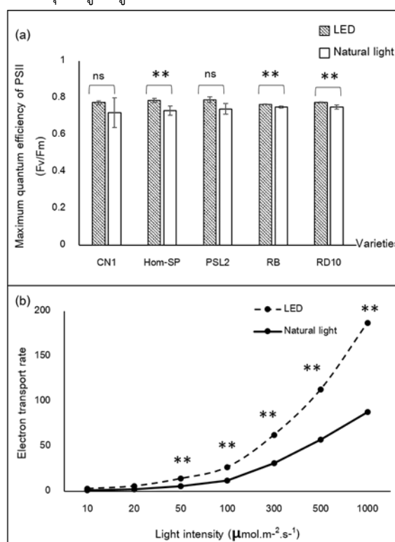
Figure 1 Maximum quantum efficiency of PSII (Fv/Fm) (a) and ETR (b) of rice leaves at tillering stage. Plants were grown under LED and natural light treatments. Leaves were placed in dark-adapted state for 30 min allowing the reaction centers to be re-oxidized. Fv/Fm and ETR were the average from five replicates \pm SE. The data shows “**” indicated significant differences at P < 0.01 between the values in LED and natural light treatments. The coefficient of variation (CV %) for Fv/Fm and ETR is 8.65% and 28.15%, respectively
