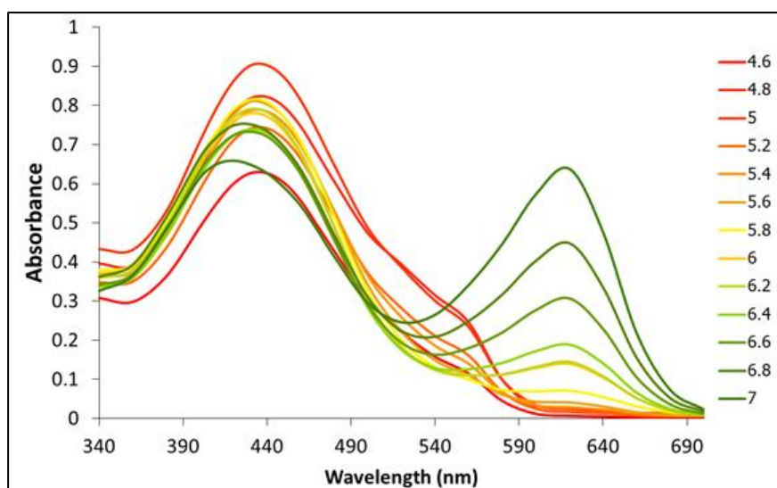
Figure 7 The absorbance of the indicator methyl red : bromothymol blue : phenolphthalein in a ratio of 1 : 2 : 1 at a pH of 4.6 to 7.0.
