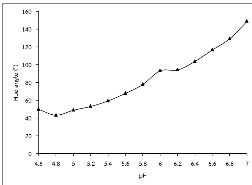
Figure 5 Hue angle (°) of indicator solution Methyl red:Bromothymol blue:Phenolphthalein in ratio 1:2:1 at pH 4.6–7.0.
