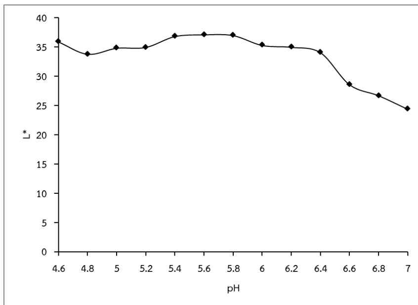
Figure 3 L* value of indicator solution Methyl red:Bromothymol blue:Phenolphthalein in ratio 1:2:1 at pH 4.6–7.0.
