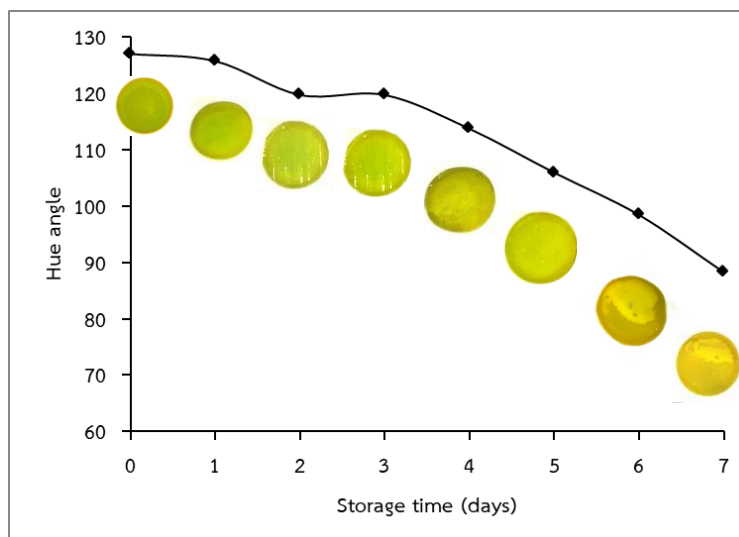
Figure 8 Hue angle of i ndicator formonitoring of fresh-cut butterhead lettuce stored at 4\pm 1^{\circ}\text{C} .
