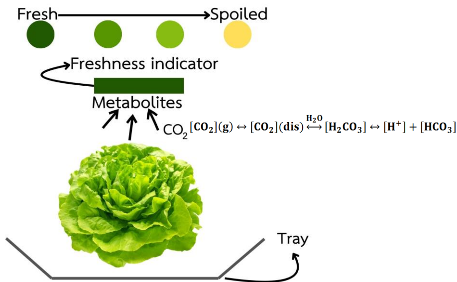
Figure 1 The mechanism of spoilage indicator.
