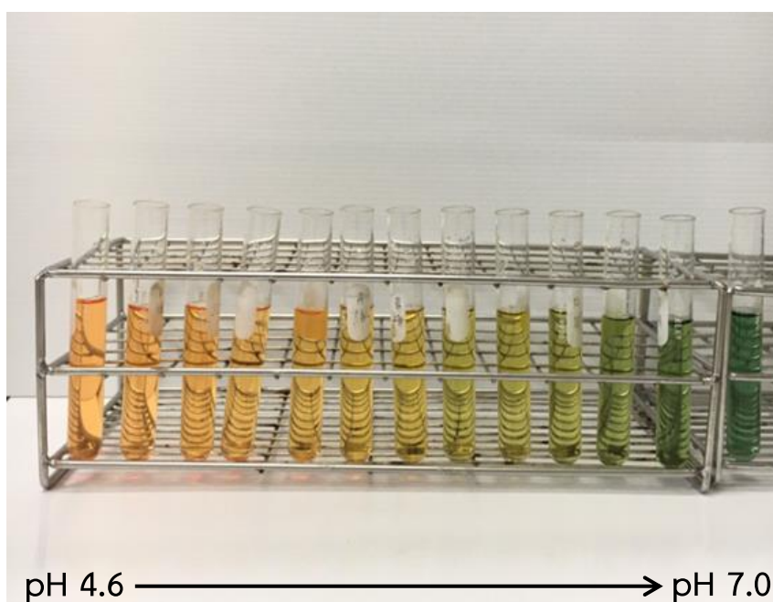
Figure 6 color changed of indicator solution methyl red:bromothymol blue:phenolphthalein in ratio 1:2:1 at pH 4.6-7.0
