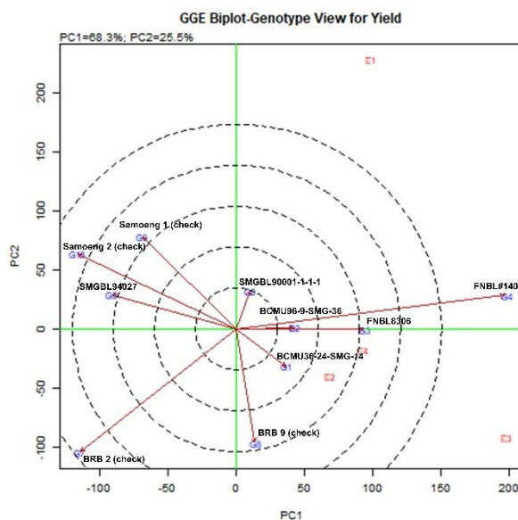
Figure 1 The genotype-vector view of GGE biplot shows similarities among 10 genotypes in their performances in individual environments in season 2022/2023
