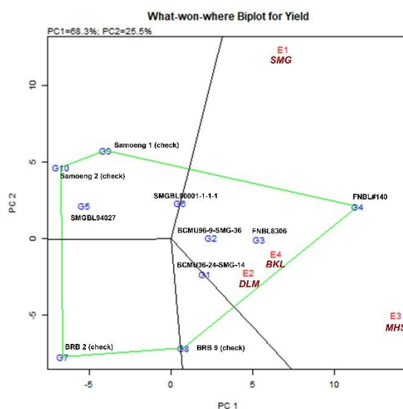
Figure 4 The which-won-where view of GGE biplot shows which genotypes performed well in which environments in season, 2022/2023
