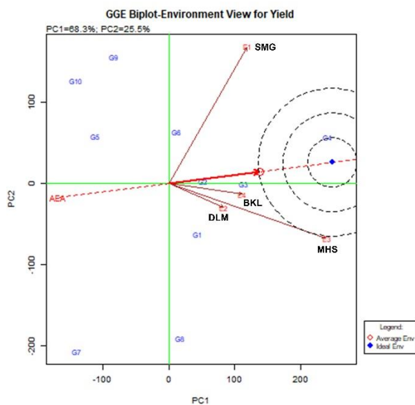
Figure 2 The discrimination and representativeness view of GGE biplot shows the discriminating ability and representativeness the Samoeng Rice Research Center, Samoeng District, Chiang Mai Province (SMG), Dong Lak Muen Experimental rice and temperate cereal, Fang District, Chiang Mai Province (DLM), Mae Hong Son Rice Research Center, Pang Mapha District, Mae Hong Son Province (MHS) and Bo Kluea Royal Project Development Project, Bo Kluea District, Nan Province (BKL) in season, 2022/2023
