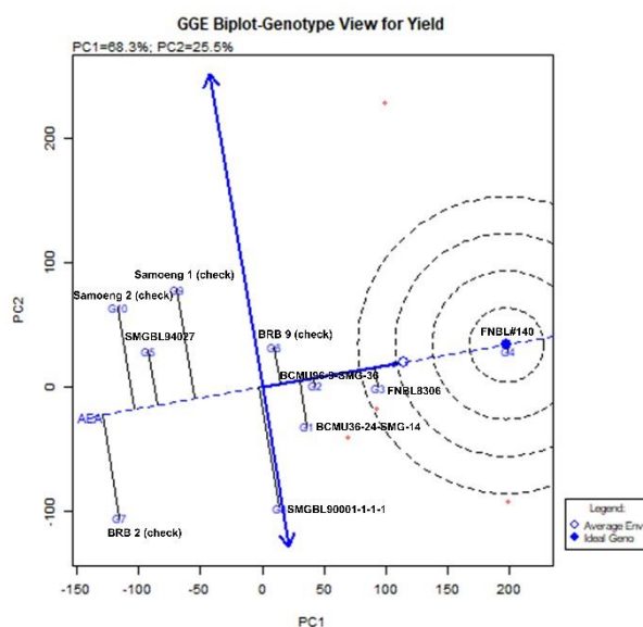
Figure 3 The average-environment axis (AEA) view of GGE biplot shows the mean performance and stability of the 10 genotypes in season, 2022/2023
