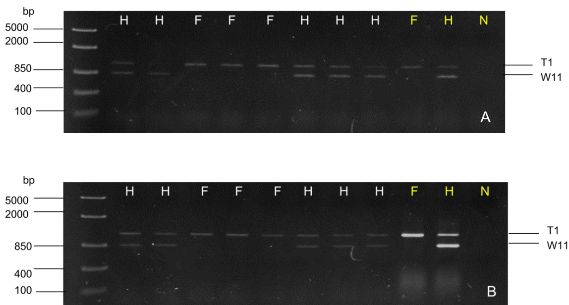
Figure 2 PCR products of T1 and W11 using two different DNA template types A) DNA from CTAB DNA extraction method and B) DNA from ground leaf tissue in NaOH; H = Hermaphrodite , F = Female and N = negative control
