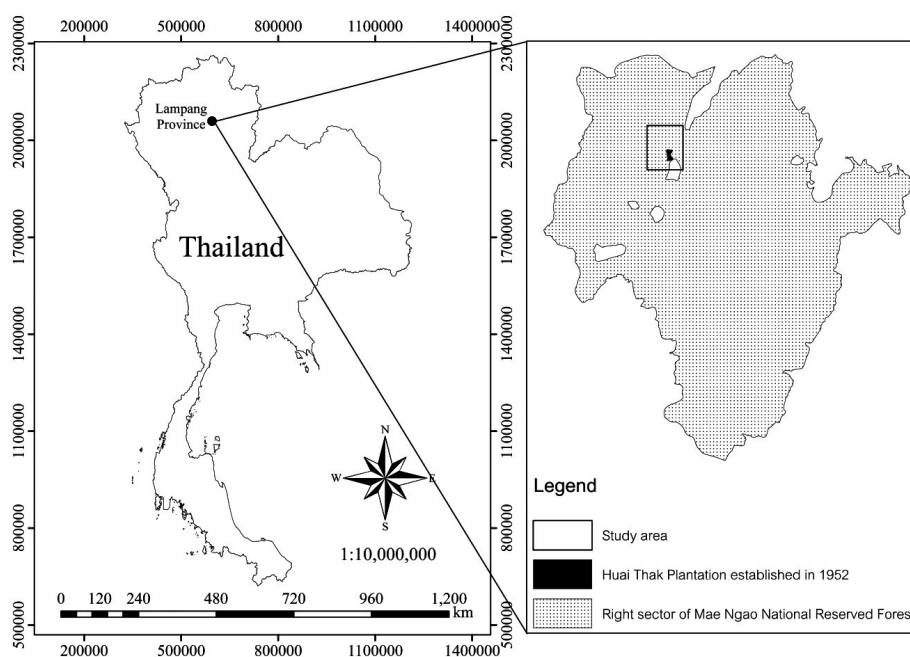
Fig. 1 Locations of study areas in natural forest (right sector of Mae Ngao National Reserved Forest) and Huai Thak plantation in Lampang province, Thailand.
