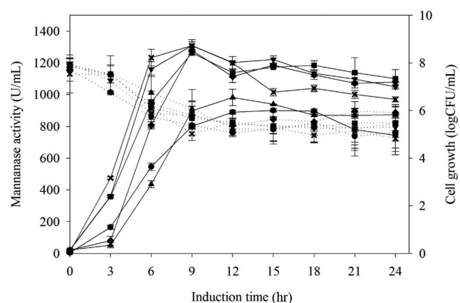
Fig. 2 Cell growth and mannanase activity after induction by 1 mM IPTG and different concentrations of lactose. Cultivations were performed in modified M9NG medium at 37°C. (.....) represents cell growth and (—) represents mannanase activity induced with 1 mM IPTG (●), 1 mM lactose (▲), 5 mM lactose (■), 10 mM lactose (▼), 15 mM lactose (×) and 20 mM lactose (○).
