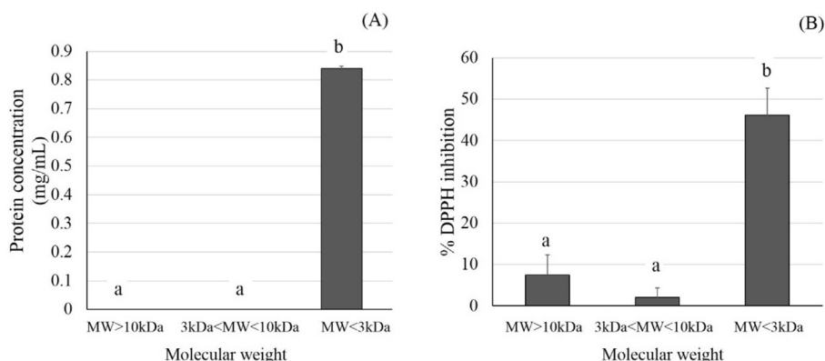
Fig. 3. (A) Molecular weight of proteins in fraction 2; (B) percentage 2,2-diphenyl-1-picrylhydrazyl (DPPH) inhibition activity of proteins in fraction 2, where each bar represents mean \pm SD ( n = 3 ) and different lowercase letters represent significant ( p < 0.05 ) differences among means.
