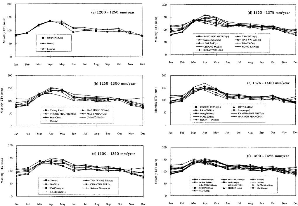
Figure 1 Monthly potential evapotranspiration of Thailand based on Penman-Monteith’s formula. (a) = agroclimatological station (c) = climatological station.
