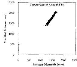
Figure 3 Comparison of annual ETo calculated by Penman-Monteith and Modified Penman formulas.
