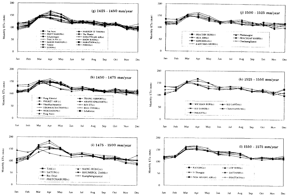
Figure 1 (cont'd) Monthly potential evapotranspiration of Thailand based on Penman-Monteith's formula. (a) = agroclimatological station (c) = climatological station
