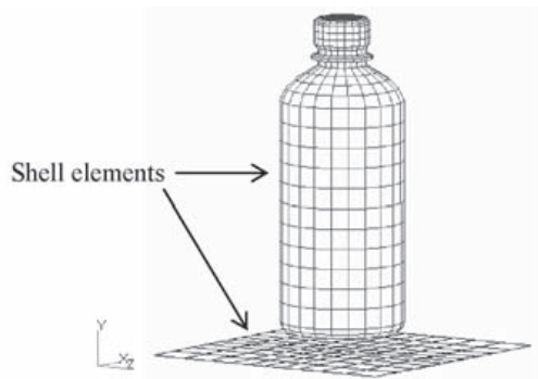
Figure 11 The bottle and force plate models.
