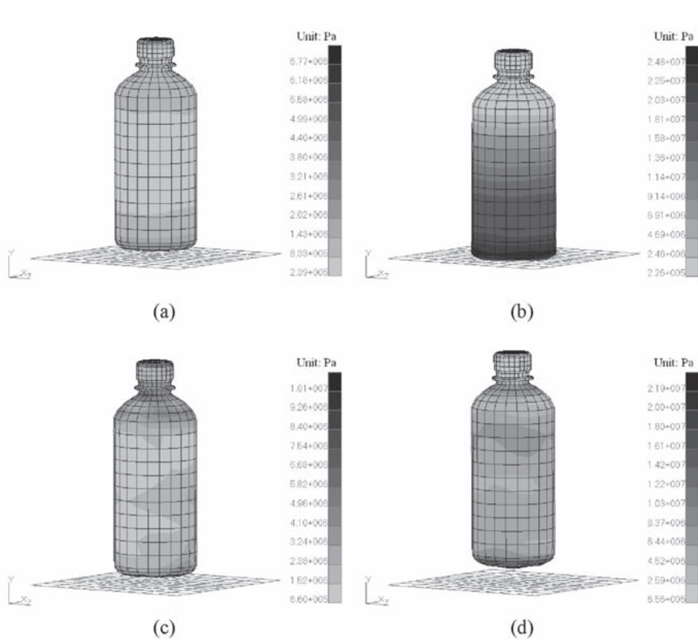
Figure 23 The contour plot of von misses stress obtained from case III (1.0 m drop height) in sequent from (a) to (d) of the full water-filled bottle.
