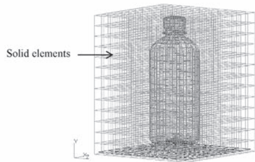
Figure 12 The fluid models.
