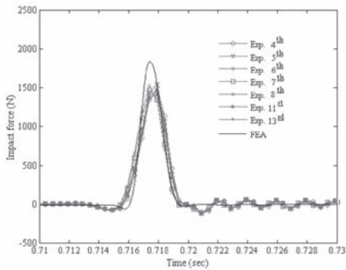
Figure 19 Force traces of the drop test of half water-filled bottles from 1.5 meter height comparing FEA with experiment.
