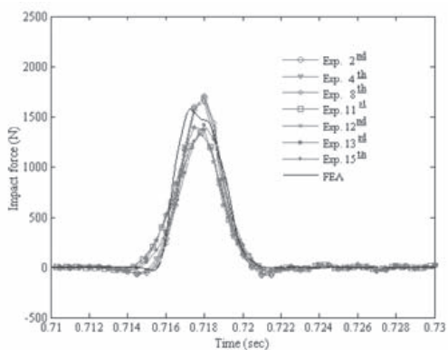
Figure 21 Force traces of the drop test of full water-filled bottles from 1.0 meter height comparing FEA with experiment.
