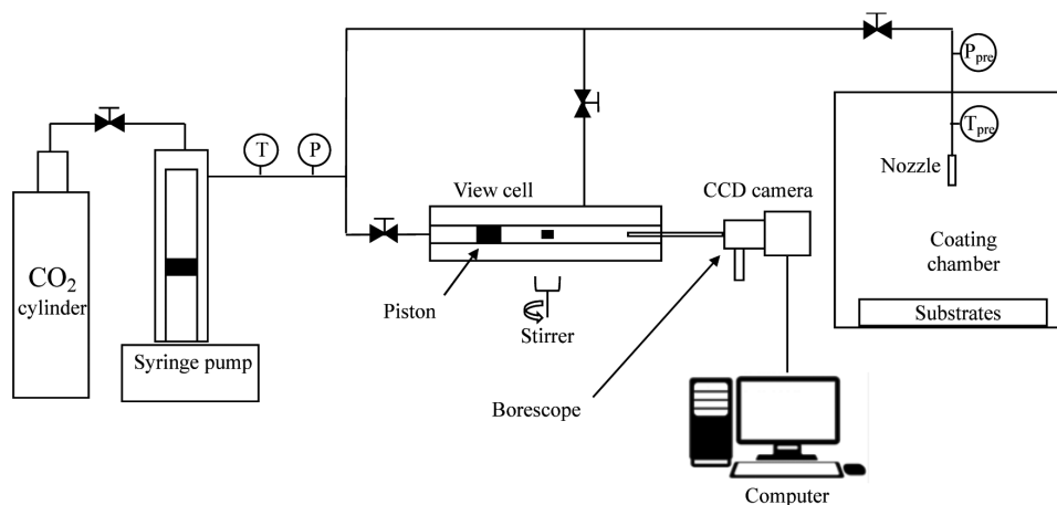
Fig. 1 Schematic of the phase behavior and apparatus for rapid expansion of subcritical solutions
