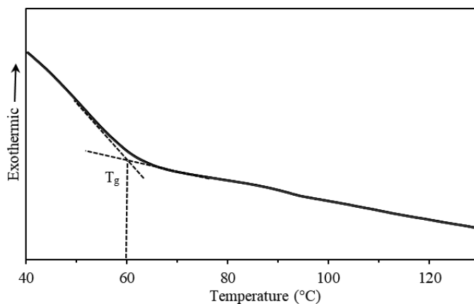
Fig. 3 Differential scanning calorimeter thermogram of lignin, where T_g = glass transition temperature
