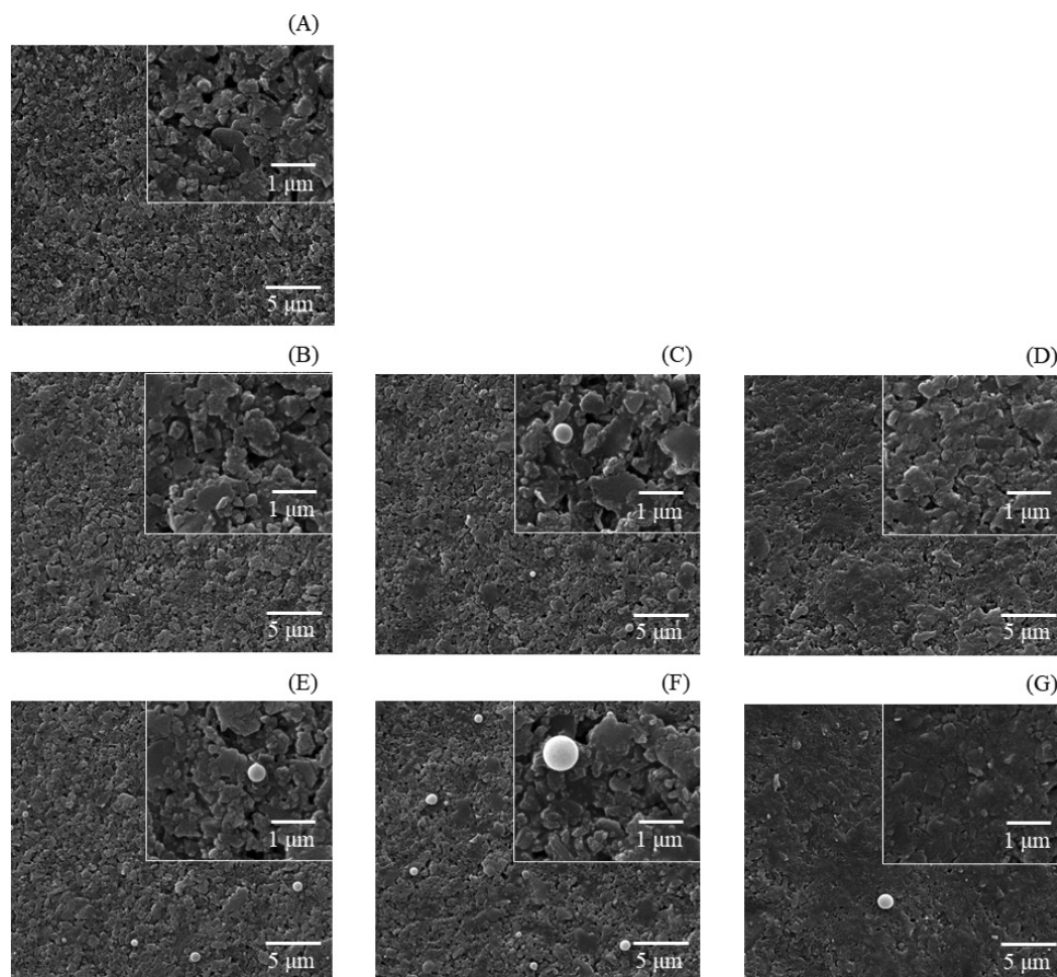
Fig. 4 Scanning electron microscope images with different values for lignin content in the coating, pre-expansion temperature ( T_{pre} ) and pre-expansion pressure ( P_{pre} ): (A) uncoated paperboard; (B) 0.25% lignin, T_{pre} = 80^{\circ}\text{C} , P_{pre} = 24.2 MPa; (C) 0.25% lignin, T_{pre} = 100^{\circ}\text{C} , P_{pre} = 24.2 MPa; (D) 0.25% lignin, T_{pre} = 100^{\circ}\text{C} , P_{pre} = 13.8 MPa; (E) 0.50% lignin, T_{pre} = 80^{\circ}\text{C} , P_{pre} = 24.2 MPa; (F) 0.50% lignin, T_{pre} = 100^{\circ}\text{C} , P_{pre} = 24.2 MPa; (G) 0.50% lignin, T_{pre} = 100^{\circ}\text{C} , P_{pre} = 13.8 MPa
