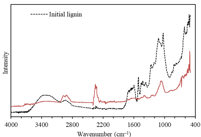
Fig. 5 Fourier transform infrared spectra of initial lignin and lignin-coated tinplate obtained from rapid expansion of subcritical solutions of 0.50% lignin at pre-expansion temperature = 100^{\circ}\text{C} and pre-expansion pressure = 13.8 MPa
