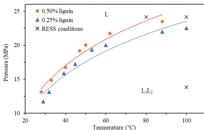
Fig. 2 Cloud-point curves for 0.25% and 0.50% lignin solutions in subcritical mixture of CO 2 + ethanol (1:1) and experimental conditions for rapid expansion of subcritical solutions (RESS) for lignin coatings in relation to their relevant cloud-point curves, where L = lignin homogeneous liquid solution and L 1 L 2 = solvent-rich and solute-rich phases
