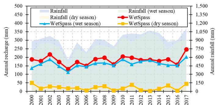
Fig. 11 Seasonal recharges based on water and energy transfer between soil, plants and atmosphere under quasi steady state (WetSpass) model
