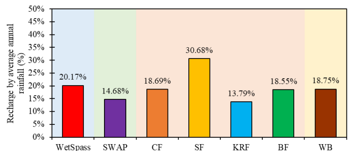
Fig. 8 Average annual recharge expressed as a percentage of average annual rainfall, where WetSpa = water and energy transfer between soil, plants and atmosphere under quasi steady state; SWAP = annual soil water atmosphere plant; CF = Chaturvedi formula; SF = Sehgal formula; KRF = Krishna Rao formula; BF = Bhattacharya formula; WB = water balance-based approach
