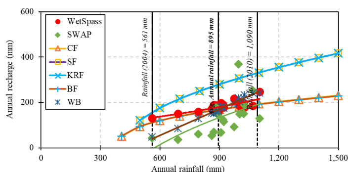
Fig. 9 Relationship of annual groundwater recharges and annual rainfall, where WetSpass = water and energy transfer between soil, plants and atmosphere under quasi steady state; SWAP = annual soil water atmosphere plant; CF = Chaturvedi formula; SF = Sehgal formula; KRF = Krishna Rao formula; BF = Bhattacharya formula; WB = water balance-based approach
