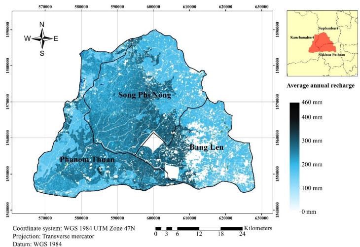
Fig. 6 Spatial distribution of average annual water and energy transfer between soil, plants and atmosphere under quasi steady state (WetSpss) recharges during 2000–2017
