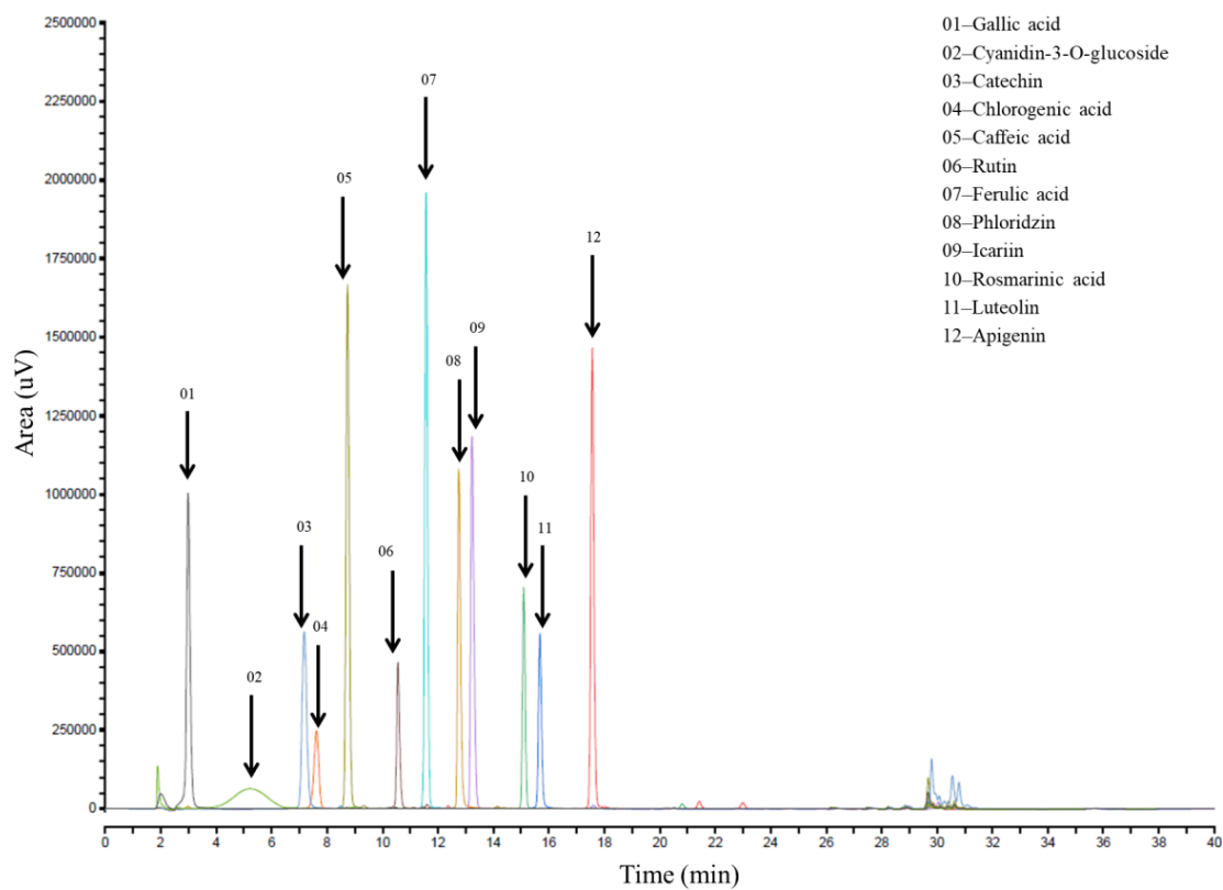
Fig. S2 Chromatogram of 12 antioxidant standards as retention time references for compound identification of metabolites produced by isolated fungi
