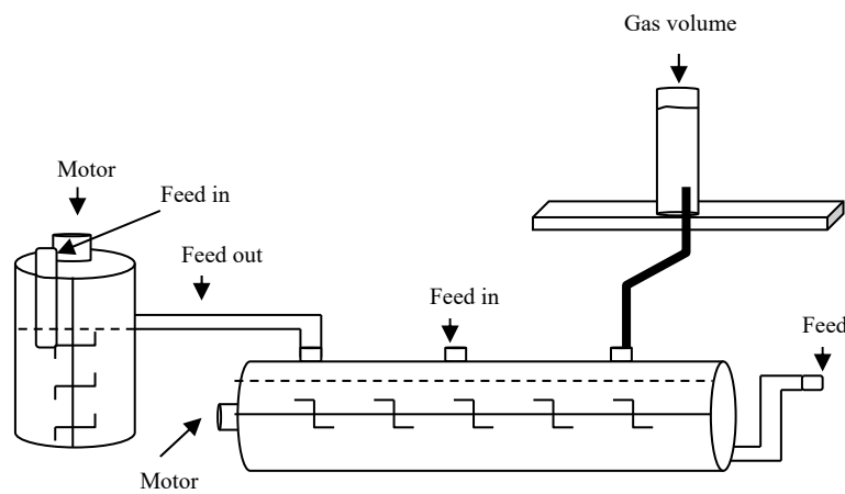
Figure 1 Diagram of two phase fermentation tank
