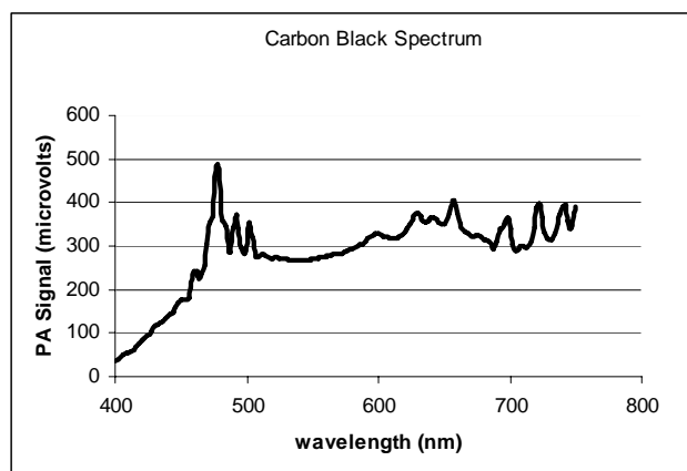
Figure 2 PA Spectrum of standard sample (carbon black).
