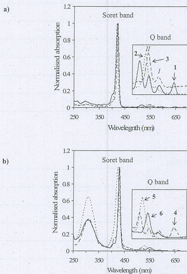
Figure 4 Normalised UV-Visible absorption spectra of a) G-0 porphyrins; b) G-1 porphyrins in dichloromethane (10 -5 M)
