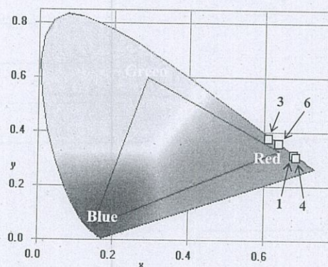
Figure 6 CIE coordinate of the porphyrin dendrimers
