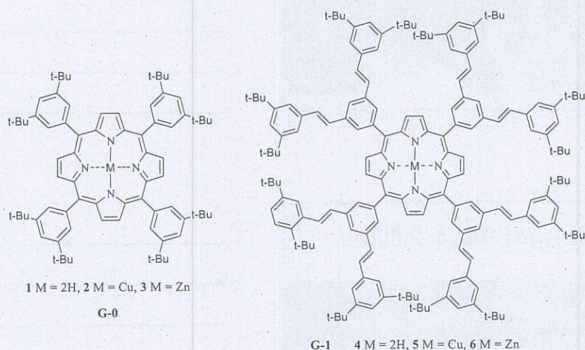
Figure 1 Molecular structures of porphyrin dendrimers
