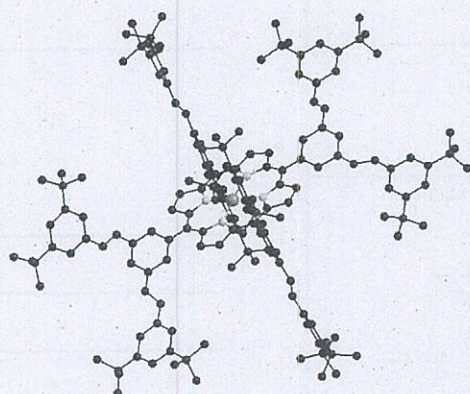
Figure 2 The optimised molecular structure of the G-1 zinc porphyrin 6
