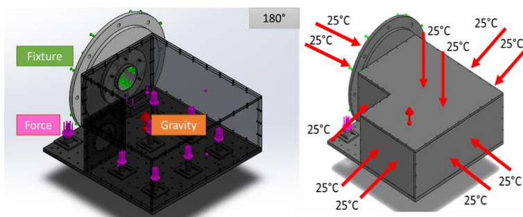
Figure 6. Left-hand panel: Assumptions used for the calculation of the mechanical deformations induced by the gravity of the spectrograph at the orientation equal to 180^{\circ} . Right-hand panel: Schematic of the assumption made on the environment temperature for the calculation of the deformations induced by the thermos-elastic effect
