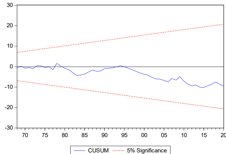
Figure 3. Stability test
