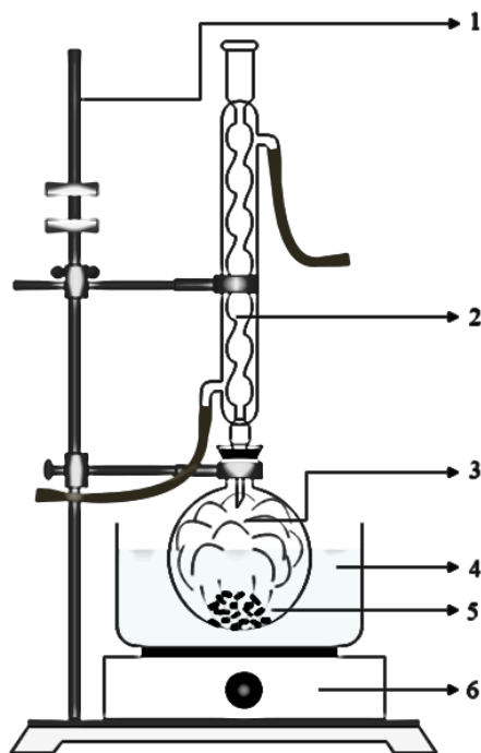
Figure 1. Reflux extraction system 1. Retort stand 2. Condenser 3. Flask 4. Water bath 5. Boiling stone 6. Heat source
