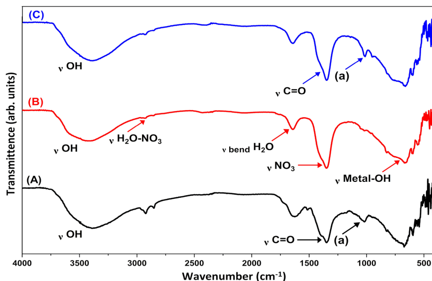
Figure 2. Full FTIR spectra of (A) N. nucifera Gaertn. flower extract, (B) Mg-Al LDH, and (C) WLE-LDH
