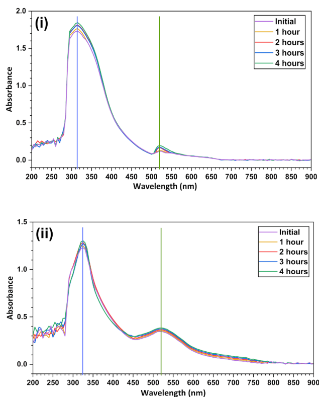
Figure 6. Absorbance spectra of DPPH radical after reduction by (i) Nelumbo nucifera Gaertn. flower crude extract and by (ii) WLE-LDH
