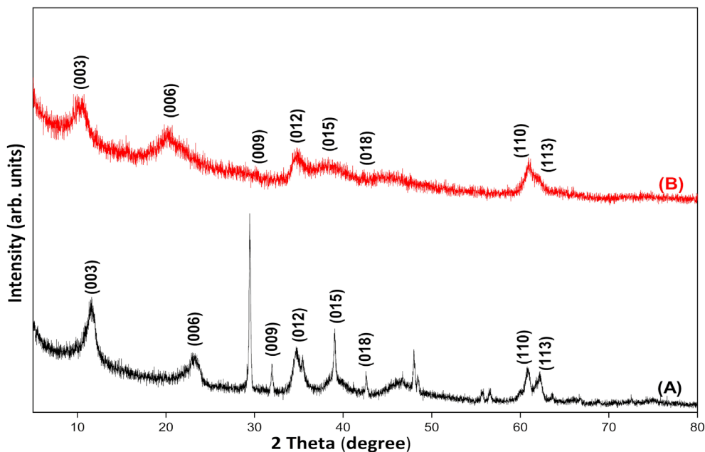
Figure 1. PXRD patterns of (A) Mg-Al LDH (B) WLE-LDH with miller indices of the planes
