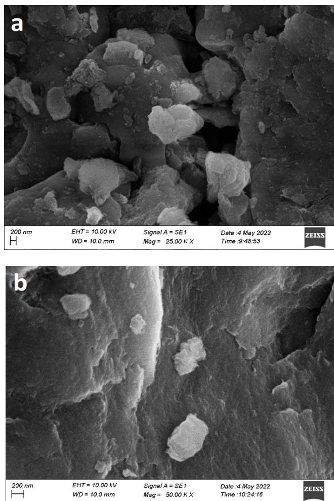
Figure 3. SEM imaging of nanomaterials (a) Pristine LDH (b) WLE-LDH. Scale bar 200 nm.
