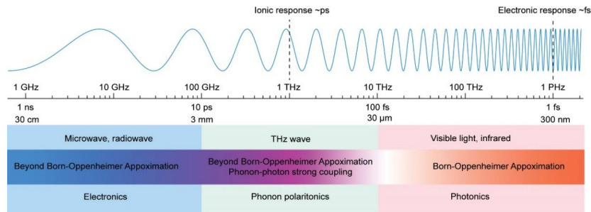
Figure 1. The dominant LMI mechanisms across the wavelength spectrum. Notably, some physical processes, including Raman/Brillouin scattering (although the pump light could be at visible or infrared wavelengths), are beyond Born–Oppenheimer approximations (Lu et al., 2024).
