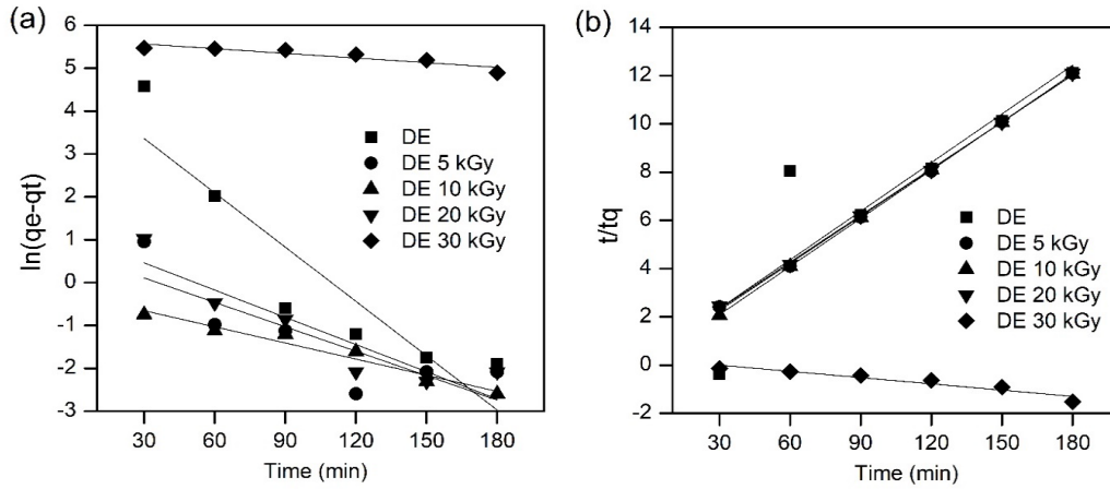
Figure 9. Kinetic model for adsorption of MB by DE and modified DE amount (a) pseudo-first order and (b) pseudo-second order
