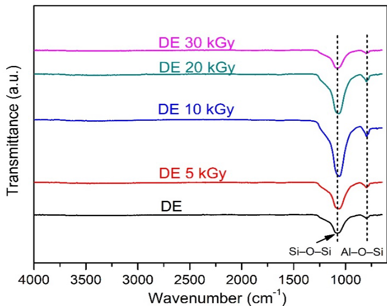
Figure 5. FT-IR spectra for the DE and modified DE
