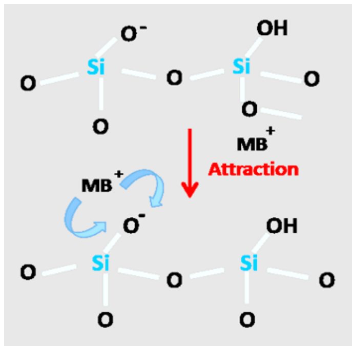
Figure 6. The possible adsorption mechanisms of MB onto DE surface
