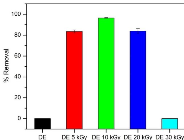
Figure 8. Effects of \gamma -irradiation on adsorption efficiency of DE and modified DE at 30 min
