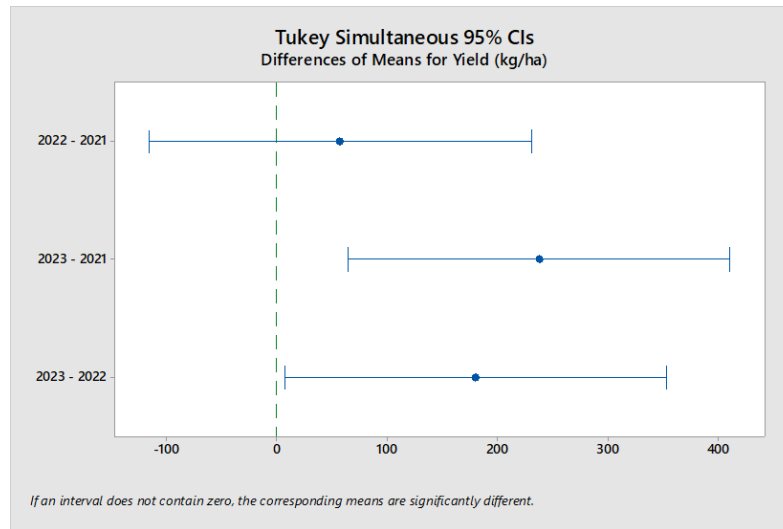
Figure2. Differences of means for yield (kg/ha)
