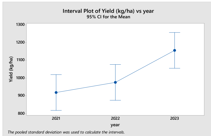
Figure 1. Interval plot of yield (kg/ha) vs year 95% CI for the mean
