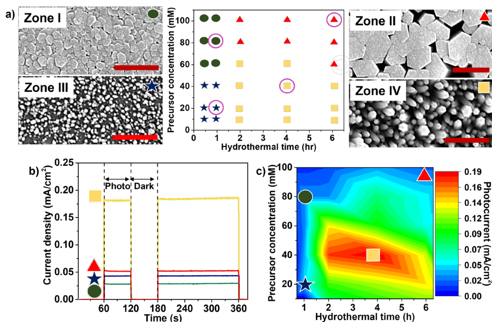
Figure 5. a) Representations of various ZnO morphologies, including dense film (zone I ●), hexagonal plates (zone II ▲), small granules (zone III ★), and nanorods (zone IV ■), obtained from varying hydrothermal parameters. b) Amperometric measurements of ZnO photoanodes with different morphologies, and c) Topographic contour of photocurrent obtained from ZnO photoanodes with various precursor concentrations and hydrothermal times (scale bar = 500 nm).
