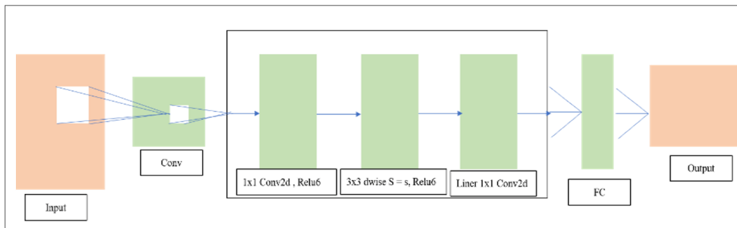
Figure 7. MobileNetV2 architecture
