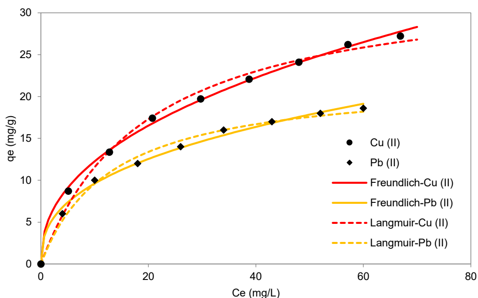
Figure 5. Equilibrium isotherm model simulations against experimental biosorption data for Cu(II) and Pb(II)
