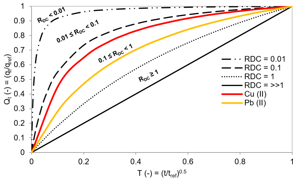
Figure 4. Typical characteristic curves of the diffusion-chemisorption model with curves of Cu(II) and Pb(II) uptake by S. marcescens overlaid
