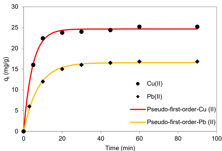
Figure 2. Pseudo-first-order kinetic model simulation of Cu(II) and Pb(II) uptake by S. marcescens . Data points represent mean values from triplicate runs \pm standard deviation (SD).
