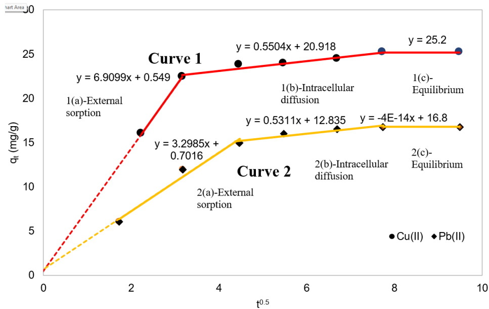
Figure 3. Plot of the Weber and Morris intraparticle diffusion model for Cu(II) and Pb(II) uptake by S. marcescens
