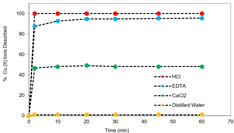
Figure 7. Desorption kinetics of Cu(II) release from S. marcescens using various eluents
