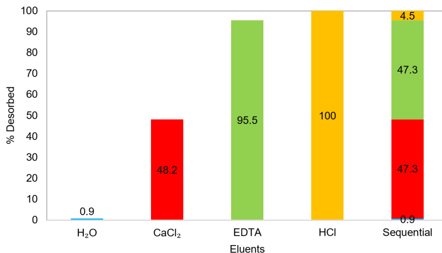
Figure 6. Cu(II) sequential and individual desorption from S. marcescens using various eluents. Bar colors correspond to the eluents tested: distilled water, CaCl 2 , EDTA and HCl.
