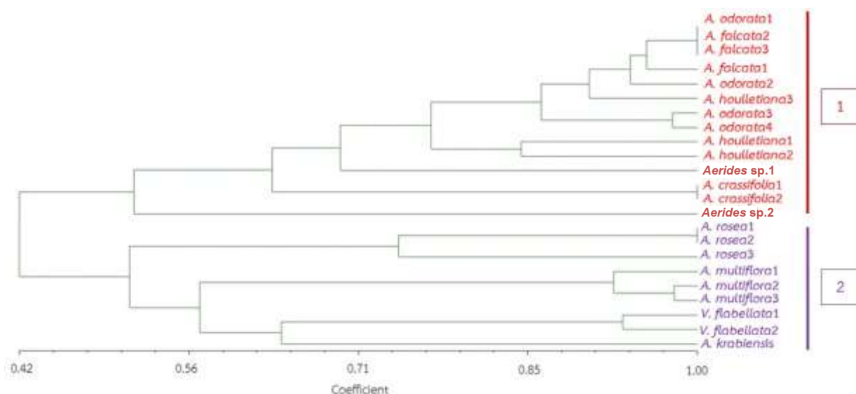
Figure 3 Dendrogram of 23 Aerides orchid samples constructed using UPGMA based cluster analysis on genetic similarities of DNA fingerprint from PCR-RFLP of cpDNA digested with Bam HI, Rsa I, Mse I, Vsp I, Hinf I, Eco RI and Taq I enzymes. Number 1 and 2 indicate two main clusters in the dendrogram.
