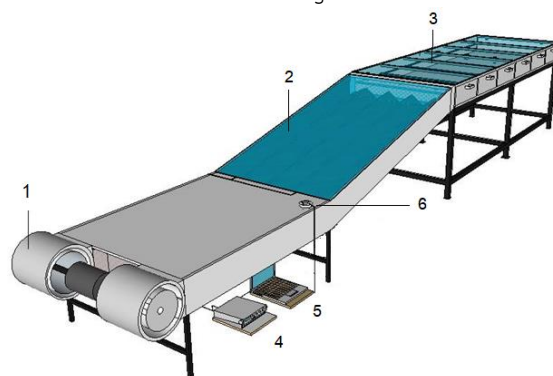
Fig. 1 A schematic diagram of the mixed-mode solar dryer: (1) Blower (2) V-grooved solar collector (3) Drying chamber (4) Data logger (5) Computer and (6) Pyranometer.
