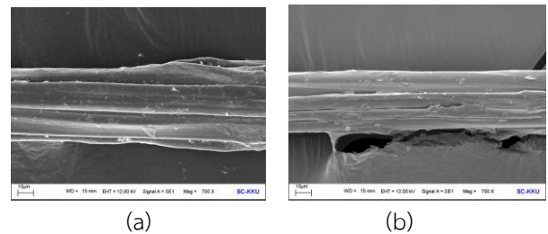
Fig. 6 Morphologies of cocoon silk: (a) Fresh cocoon and (b) Dry cocoon.
