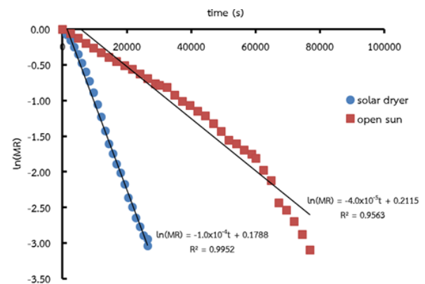
Fig. 5 Linear relationship between ln(MR) and drying time.
