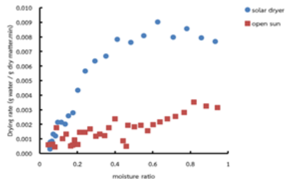
Fig. 4 Variation in drying rate versus moisture ratio.
