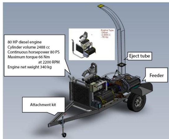
Figure 4 Preliminary drawings of the prototype system of the mobile rubber wood shredding system.
