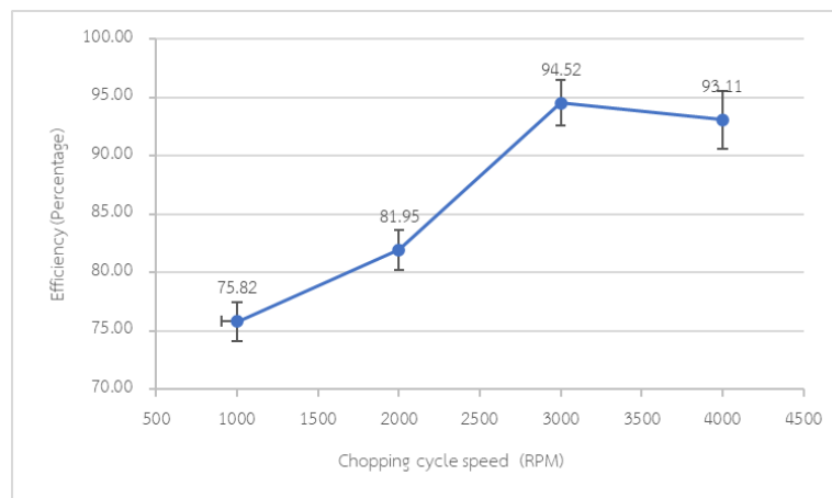
Figure 10 Relationship between chopping cycle speed and efficiency.
