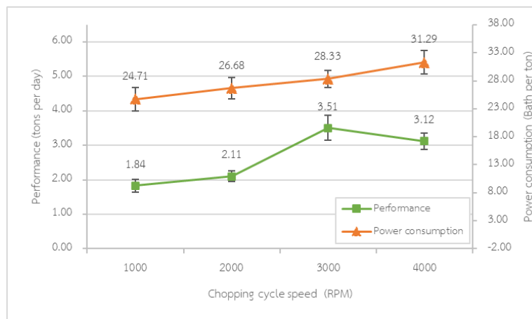
Figure 11 Relationship between chopper speed and performance and power consumption.
