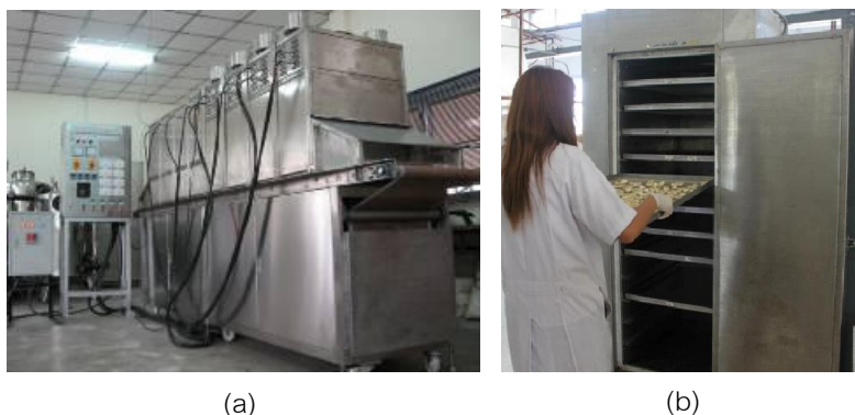
Figure 1 The continuous microwave-infrared drier which the front 4 units compose of 8 microwave magnetrons and the back units are the infrared set (a). The hot air (tray) drier used in the experiment (b). Source: Prema Asia Technology Limited.
