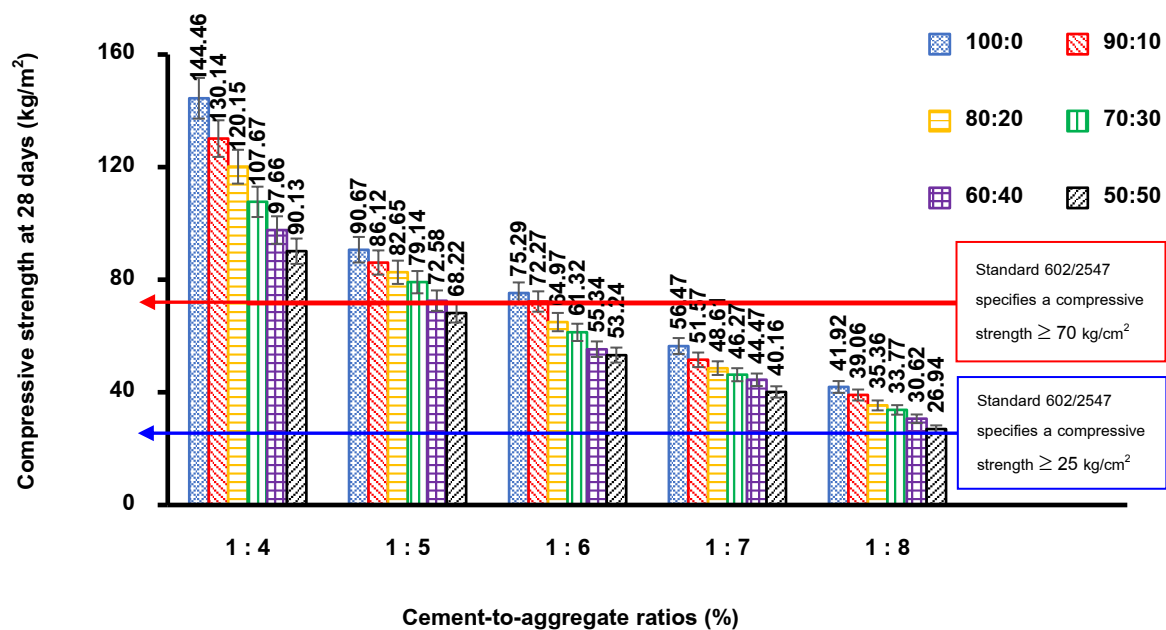
Figure 5 The effect of cement-aggregate ratio on 28-day compressive strength.
