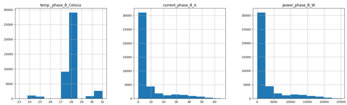
Figure 11 Histogram of temperature, current, and power for phase A.
