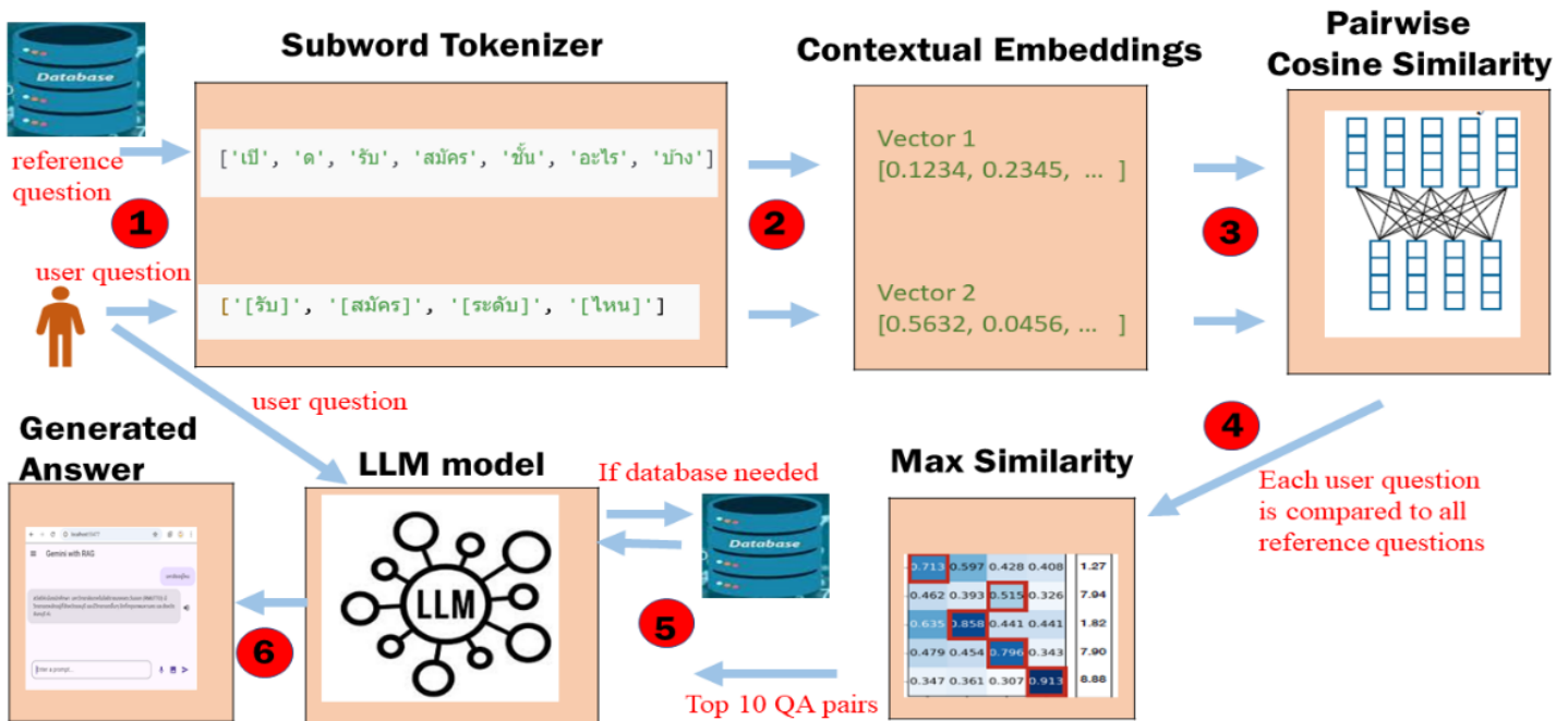
Figure 1 Over all framework of the proposed methodology.
