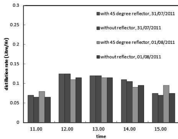
Figure 6 Distillation rate
