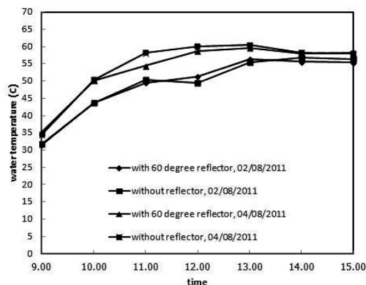
Figure 7 Water temperature
