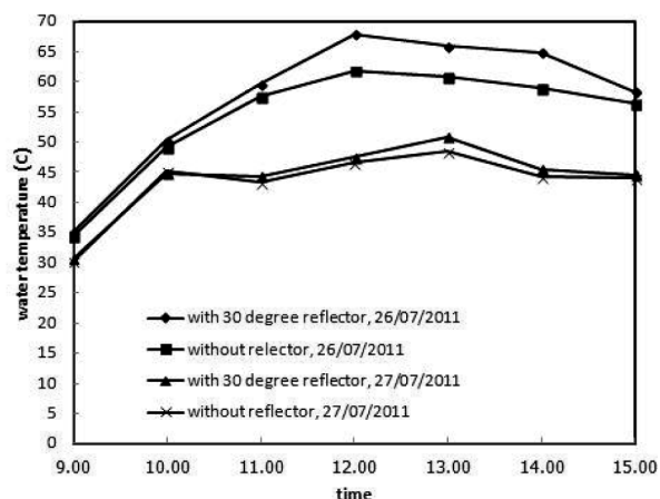
Figure 3 Water temperature
