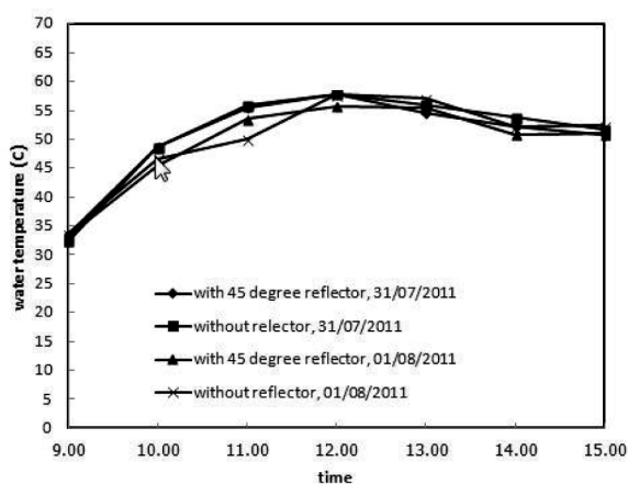
Figure 5 Water temperature
