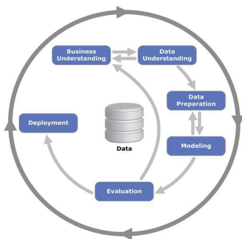
Figure 1 CRISP-DM
