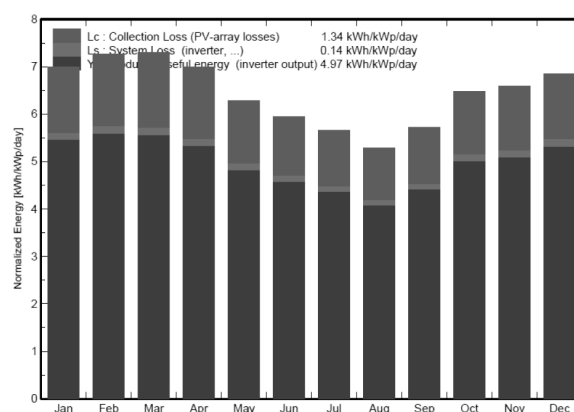
Figure 8 Performance of tracking PV system
