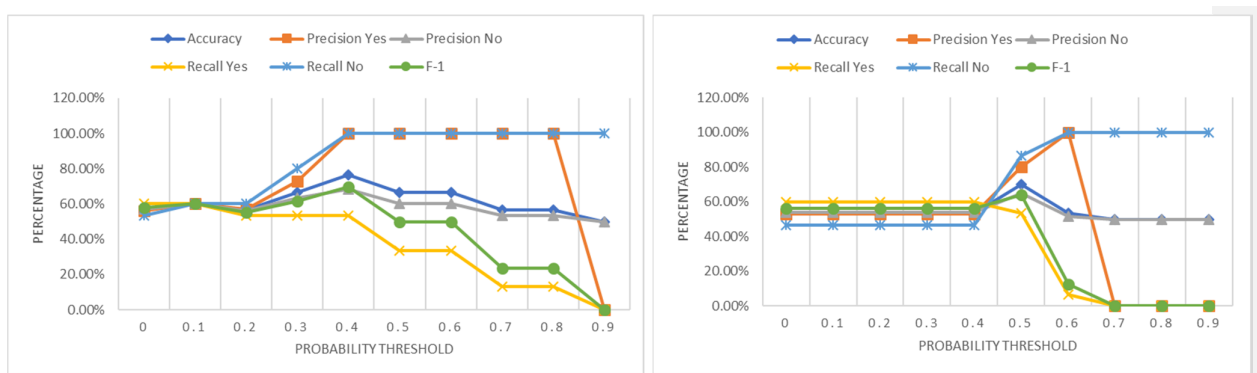
Figure 2 Performance Bayes model (Left) and SVM model (Right) by 2,000 features (1 Level)
