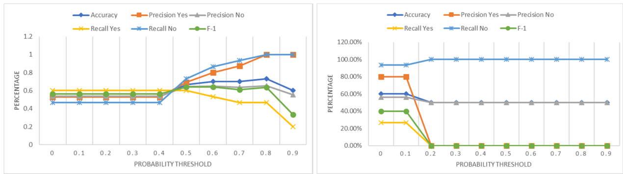
Figure 8 Performance SVM + Bayes model (Left) and SVM + Random Forest model (Right) by 6,000 features (2 Levels)
