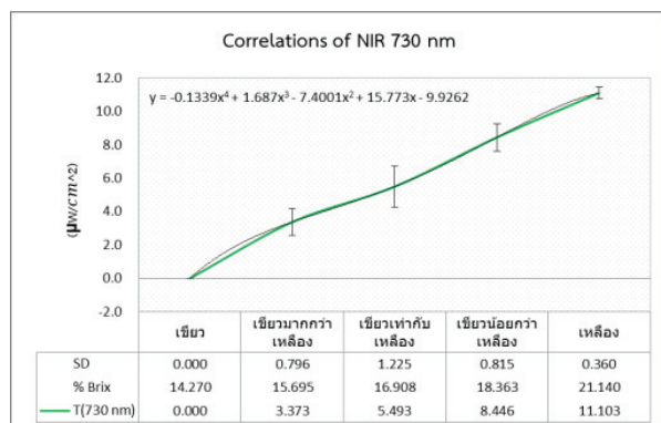
Figure 12 The 730 nm wavelength relationship of NIR with %Brix
