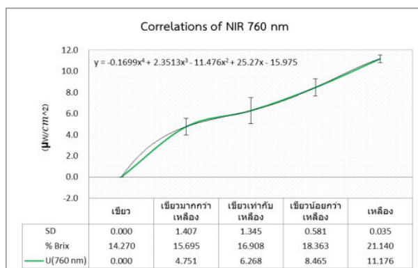
Figure 13 The 760 nm wavelength relationship of NIR with %Brix
