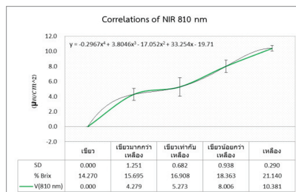
Figure 14 The 810 nm wavelength relationship of NIR with %Brix
