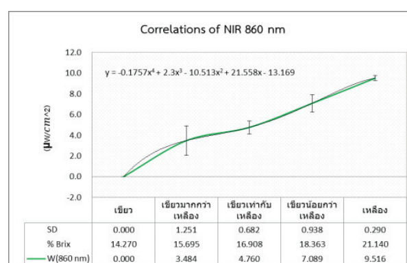
Figure 15 The 860 nm wavelength relationship of NIR with %Brix
