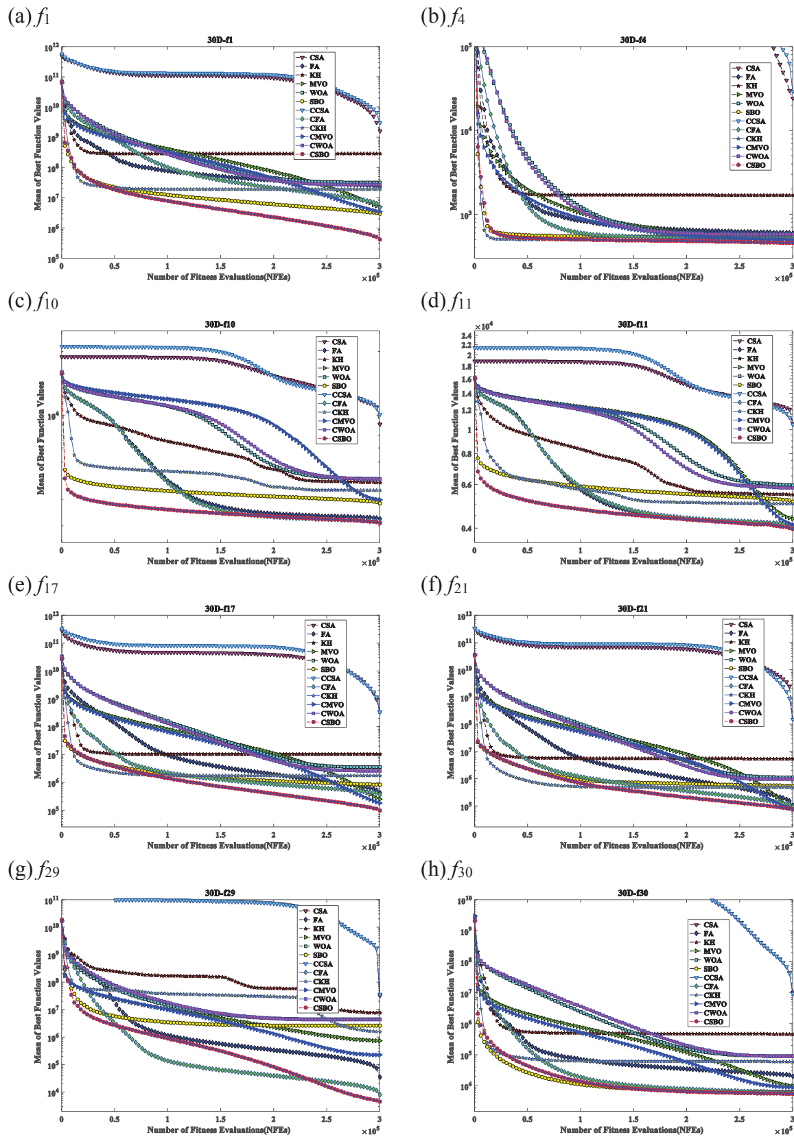
Figure 1 Convergence performance of all 12 optimization algorithms in eight benchmark functions
