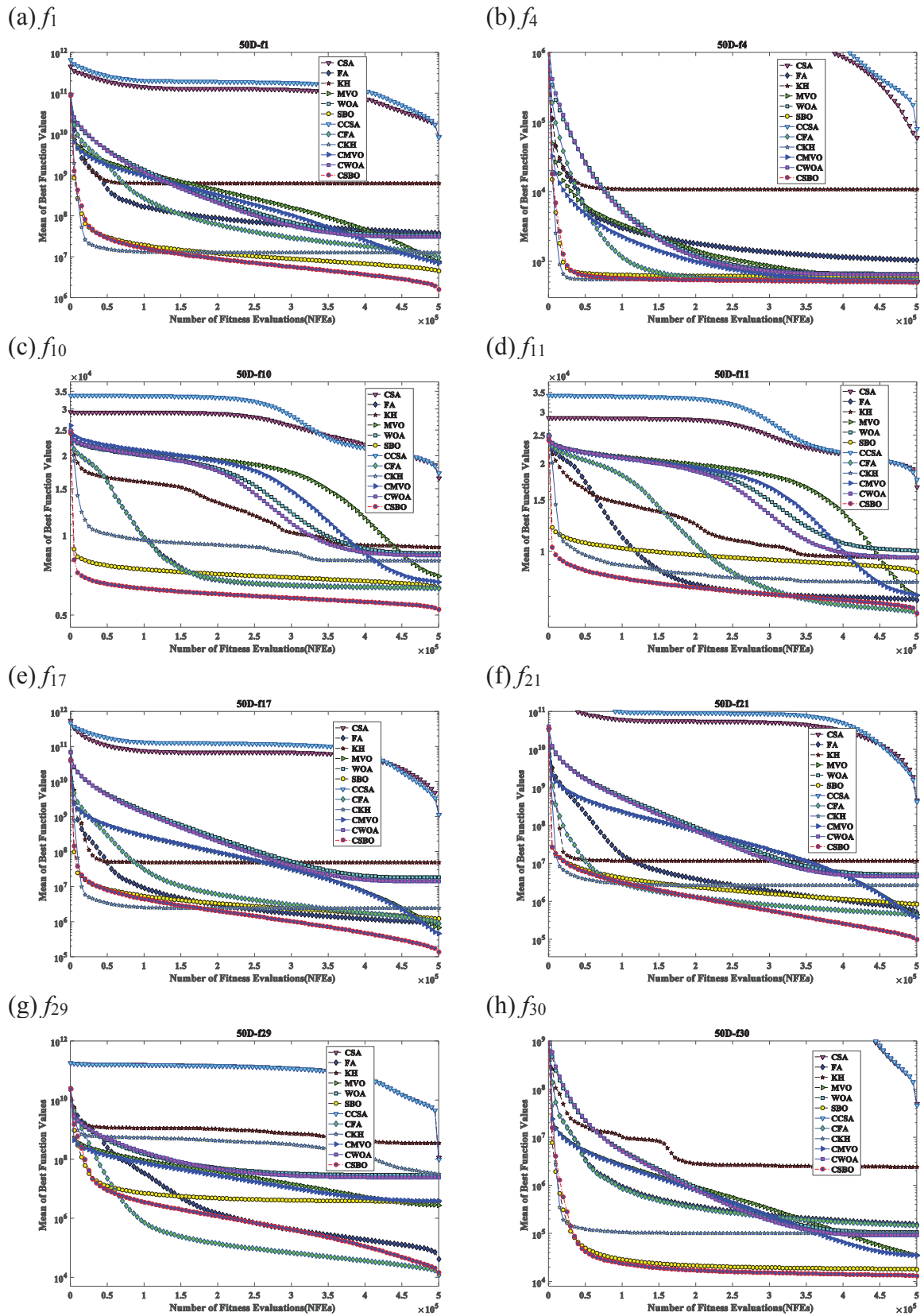
Figure 2 Convergence performance of all 12 optimization algorithms in eight benchmark functions
