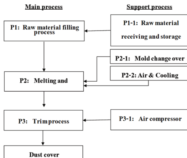
Figure 2 Show the process of manufacturing dust cover of car shock absorbers
