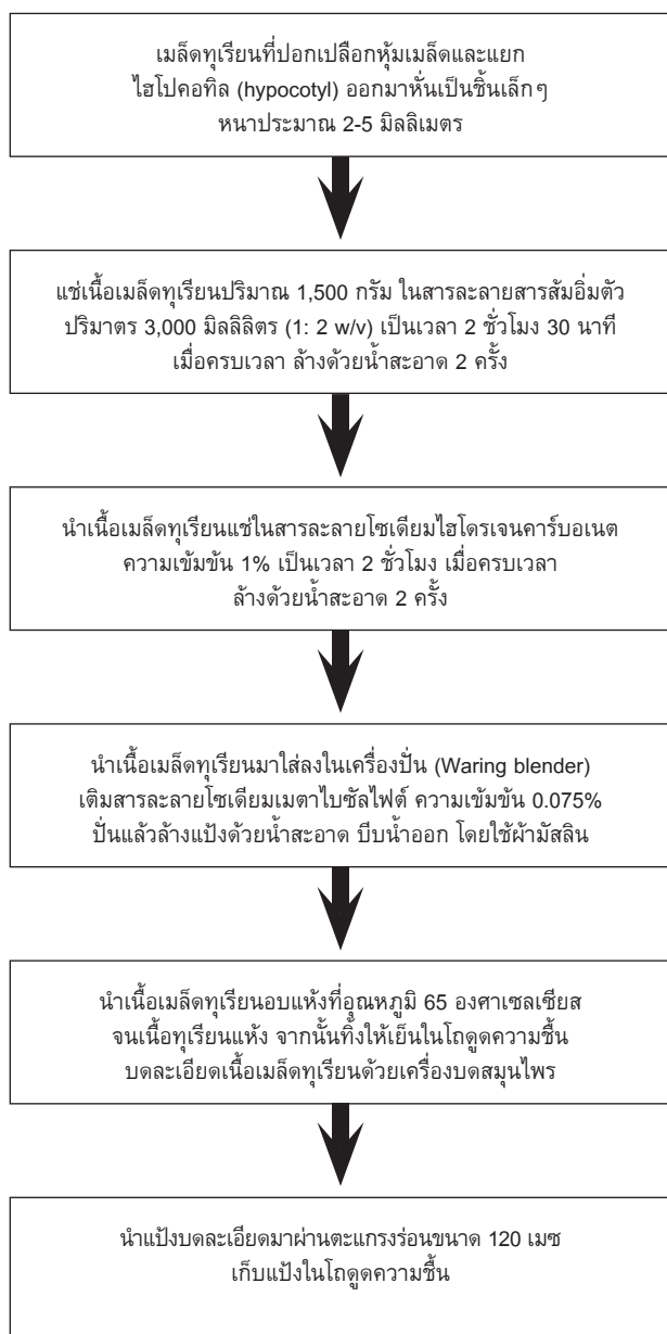
Figure 2 Method of native durian seed flour production
