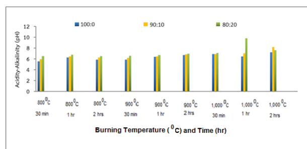
Figure 7 Acidity-Alkalinity (pH) of Lightweight Expanded Clay Aggregate
