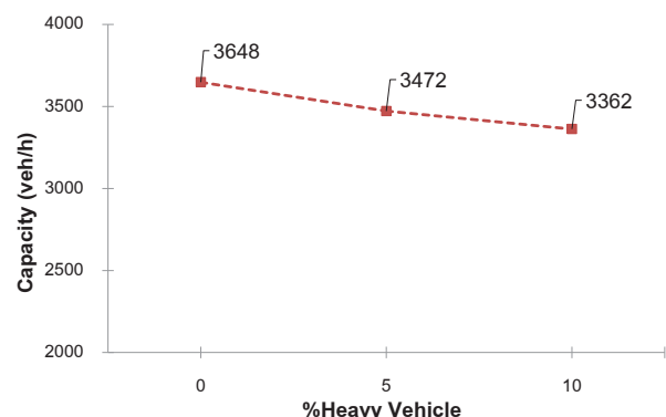
Figure 8 Impact of Heavy Vehicles on capacity for DRR two-lane highway
