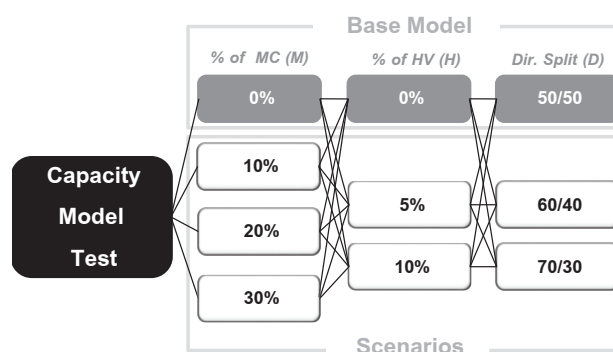
Figure 5 Scenarios test
