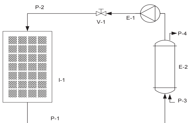
P-1 = water outlet SPVT P-2 = water inlet SPVT P-3 = water inlet storage tank P-4 = water outlet storage tank E-2 = storage tank E-1 = pump I-1 = SPVT module V-1 = screw-down valve
