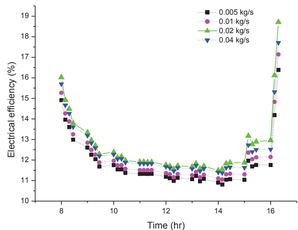
Figure 12 Electrical efficiency towards water mass flow rate
