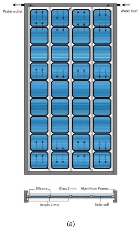
Figure 1 The cross-section SPVT module structure
