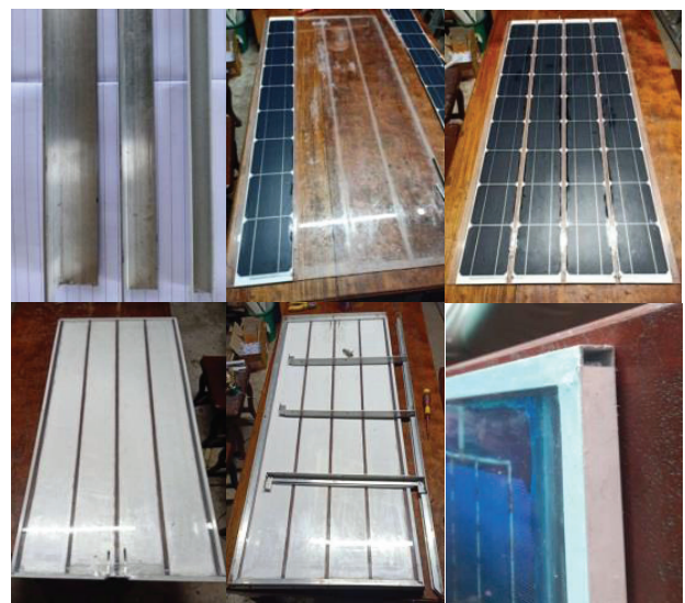
Figure 3 Construction details of the SPVT module
