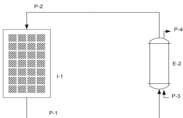
P-1 = water outlet SPVT P-2 = water inlet SPVT P-3 = water inlet storage tank P-4 = water outlet storage tank E-2 = storage tank I-1 = SPVT module
