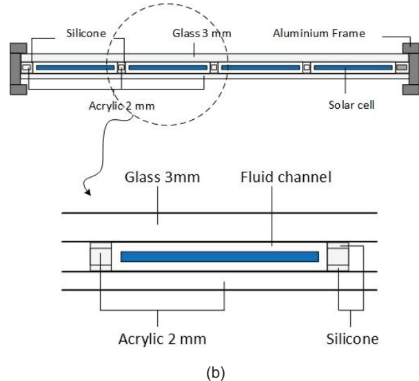
Figure 2 (a) Fluid flow diagram in the SPVT module (b) Dimension details of the SPVT module
